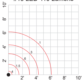
#19 LED-110 Lumens
