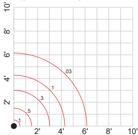
#17 LED-110 Lumens
