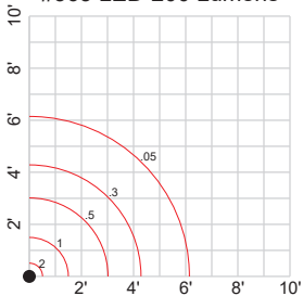
#363 LED-200 Lumens
