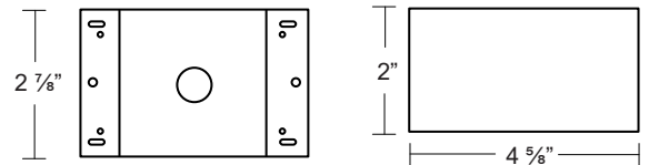
Single-gang J-Box
