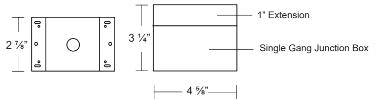
Single-gang J-Box
